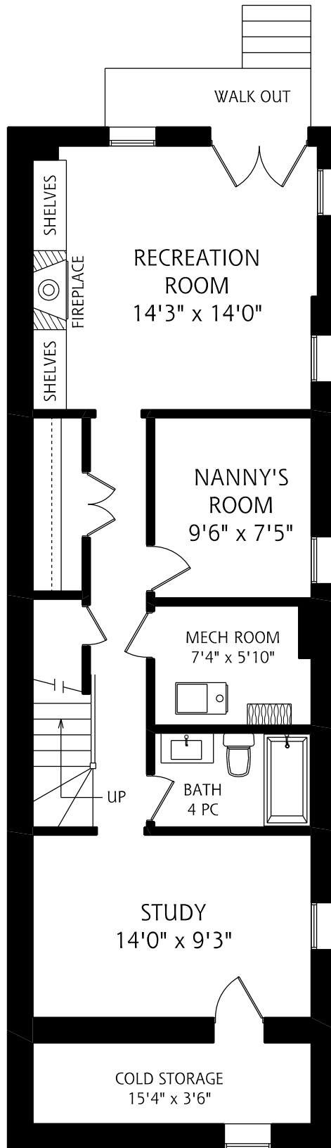
LOWER LEVEL 845 SQUARE FEET
