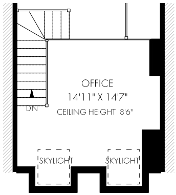
LOFT - 230 SQUARE FEET
