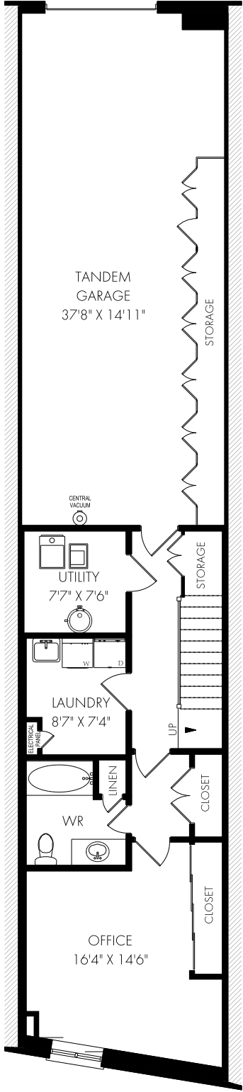
LOWER LEVEL - 618 SQUARE FEET
