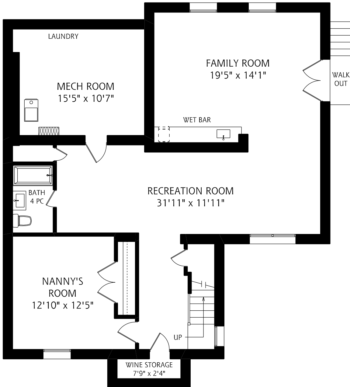
LOWER LEVEL 1,565 SQUARE FEET
