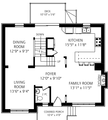
MAIN FLOOR 950 SQUARE FEET
