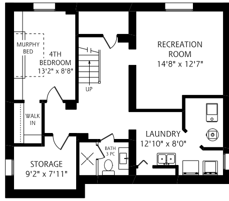
LOWER LEVEL 940 SQUARE FEET
